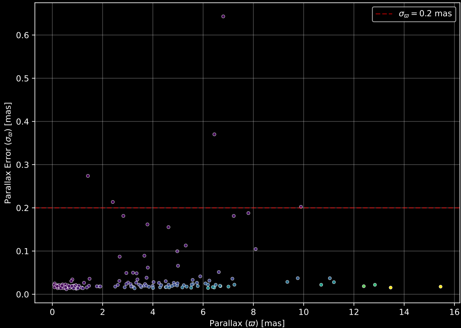
APOGEE DR17 Field: [K2_C6_331+50_btx] Parallax Quality (n= 171)
