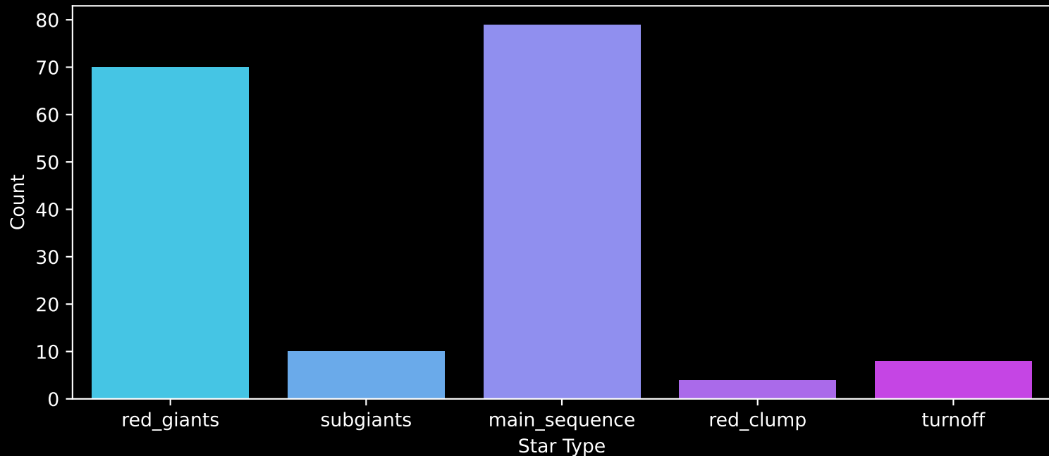
APOGEE DR17 Field: [K2_C6_331+50_btx] Count plot of Star Type
