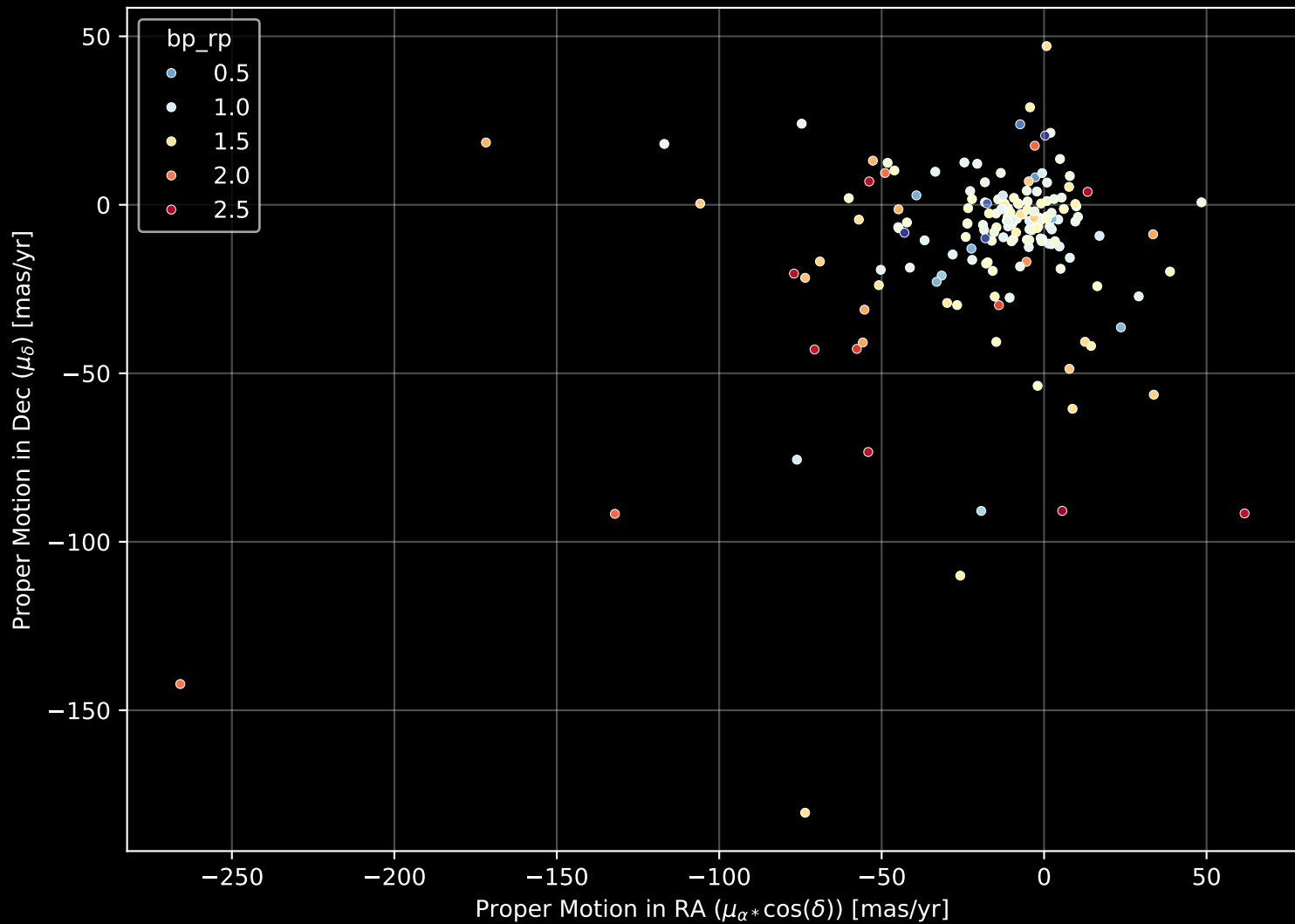
APOGEE DR17 Field: [K2_C6_331+50_btx] Proper Motion Diagram (n= 171)
