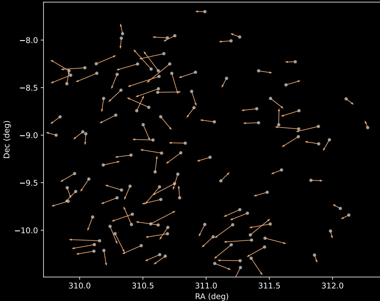
APOGEE DR17 Cluster 3 Proper Motion Vectors (n=114)
