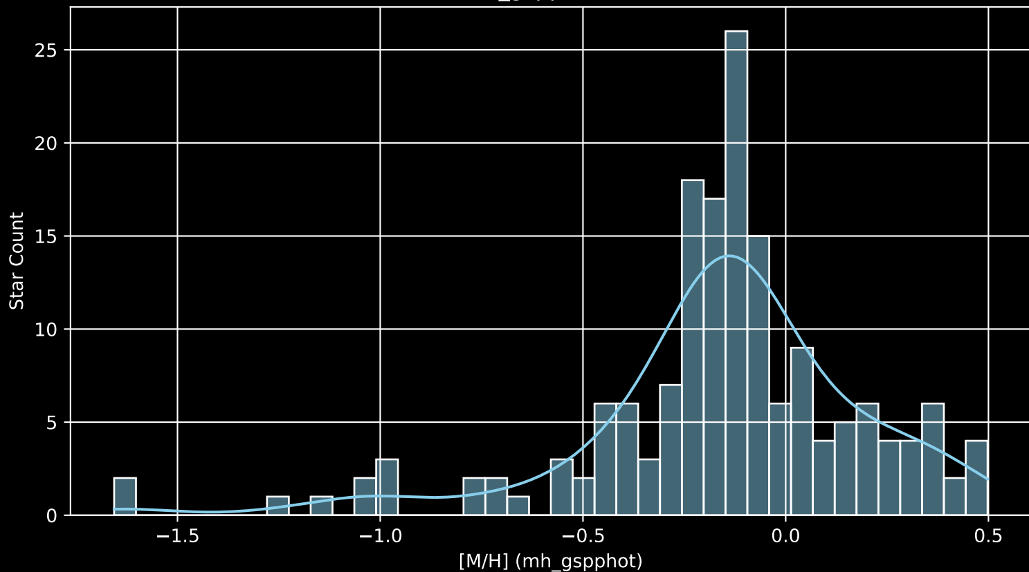
APOGEE DR17 Field: [K2_C6_331+50_btx [M/H] (mh_gspphot) (n= 167)
