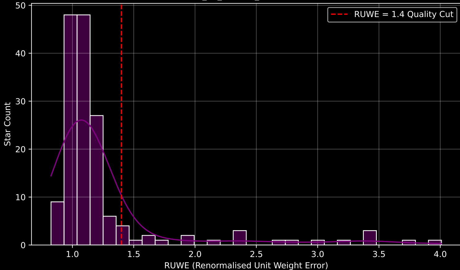
GAPOGEE DR17 Field [K2_C6_331+50_btx] RUWE Distribution (n= 161)
